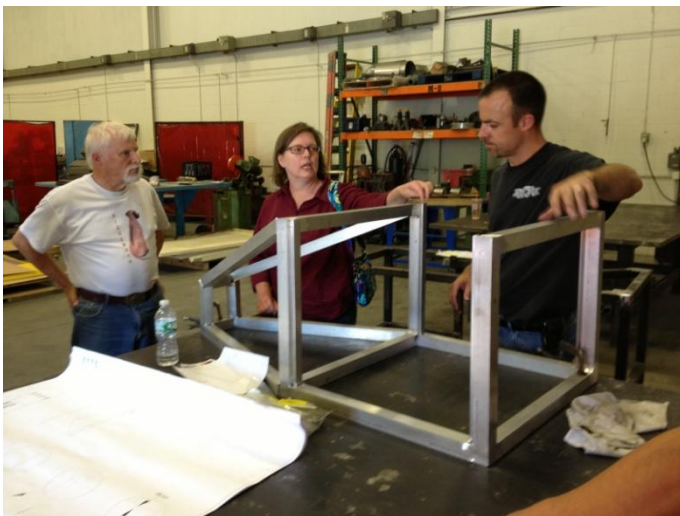
Eric Belt (volunteer) and Pat Young (Program Director for the Eightmile Wild & Scenic Partnership) confer with a craftsman from SeConn metal shop in Waterford about the design of the box that will hold the Moulson Pond Fishway camera.
