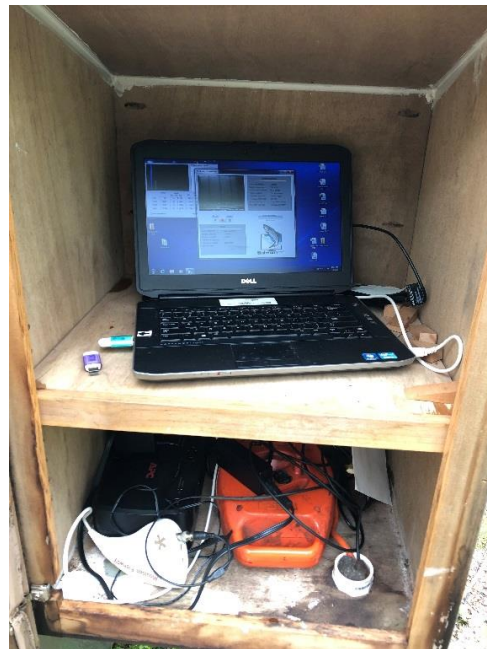
The SalmonSoft set-up for Moulson Pond. Images from an underwater camera are sent to this laptop and our crew routinely visits to download the files onto a memory stick. Files are transferred to the Cloud where volunteer Vallin reviews them and compiles data.
